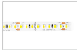
Flexiled XF24160 14.4W/m 24V DC Flexible Strip
