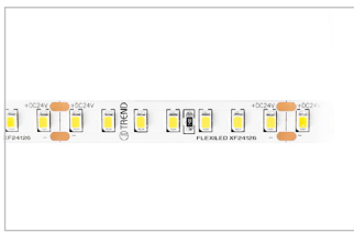
Flexiled XF24126 14.4W/m 24V DC Flexible Strip
